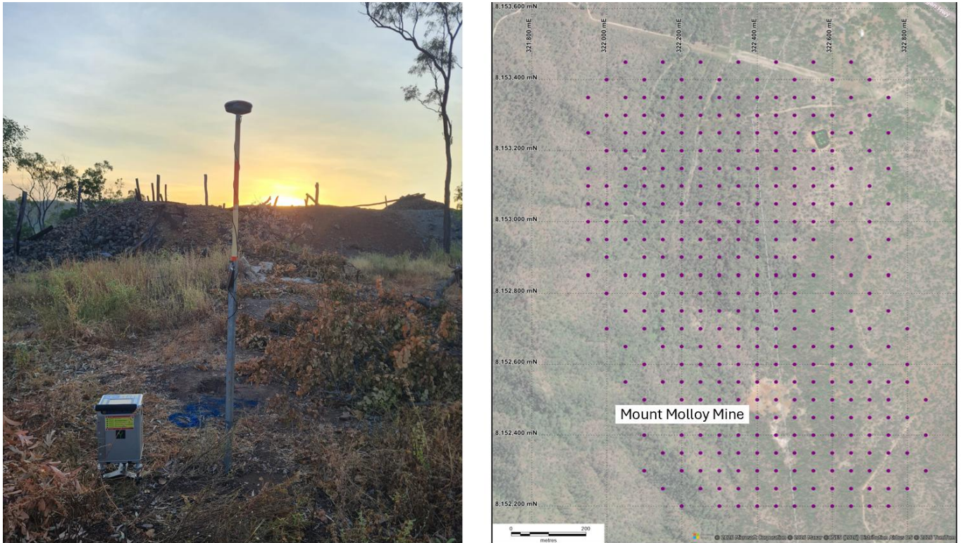
Figure 12 - Mount Molloy gravity survey
