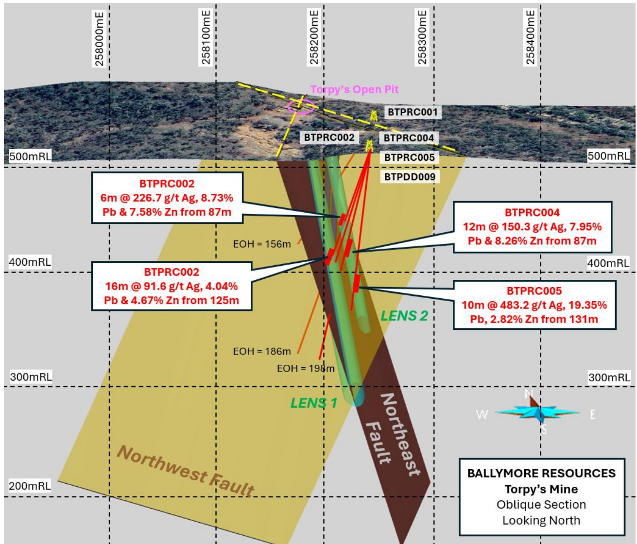
Figure 1 – Oblique section looking north towards the Torpy's prospect showing modelled northwest- and northeast-trending faults and the interpreted mineralised shoots (green) plunging moderately towards the south and the locations of drill holes BTPRC001, 002, 004 and 005 and BTPDD009.
