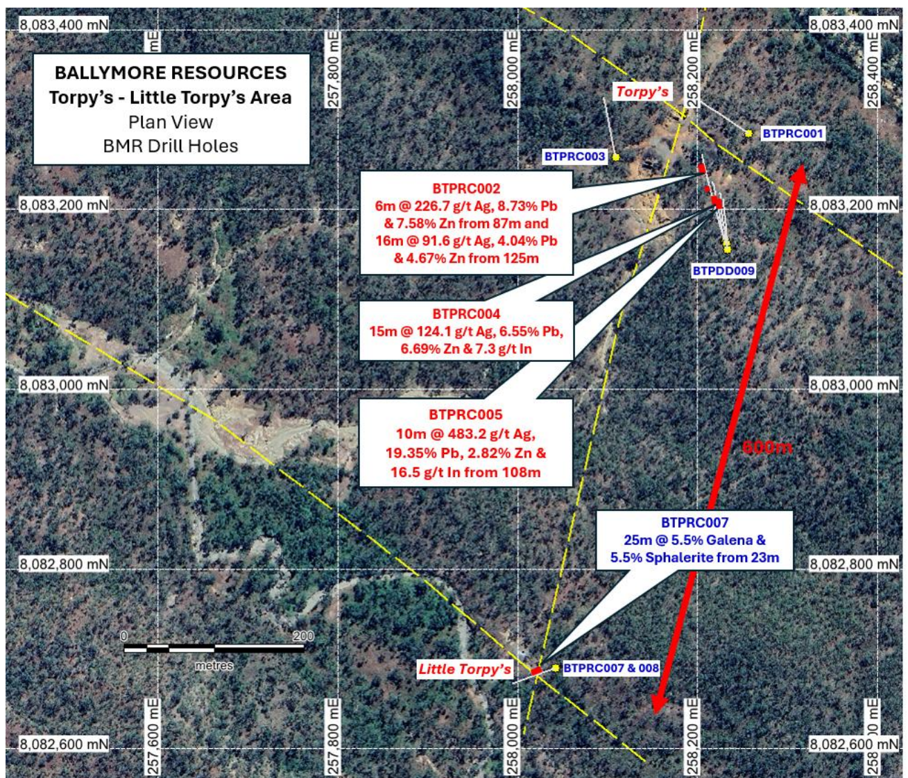
Figure 3 – Airphoto of the Torpy's - Little Torpy's area showing mapped faults (yellow) and Ballymore drill holes with assays and visual estimates of galena and sphalerite.
