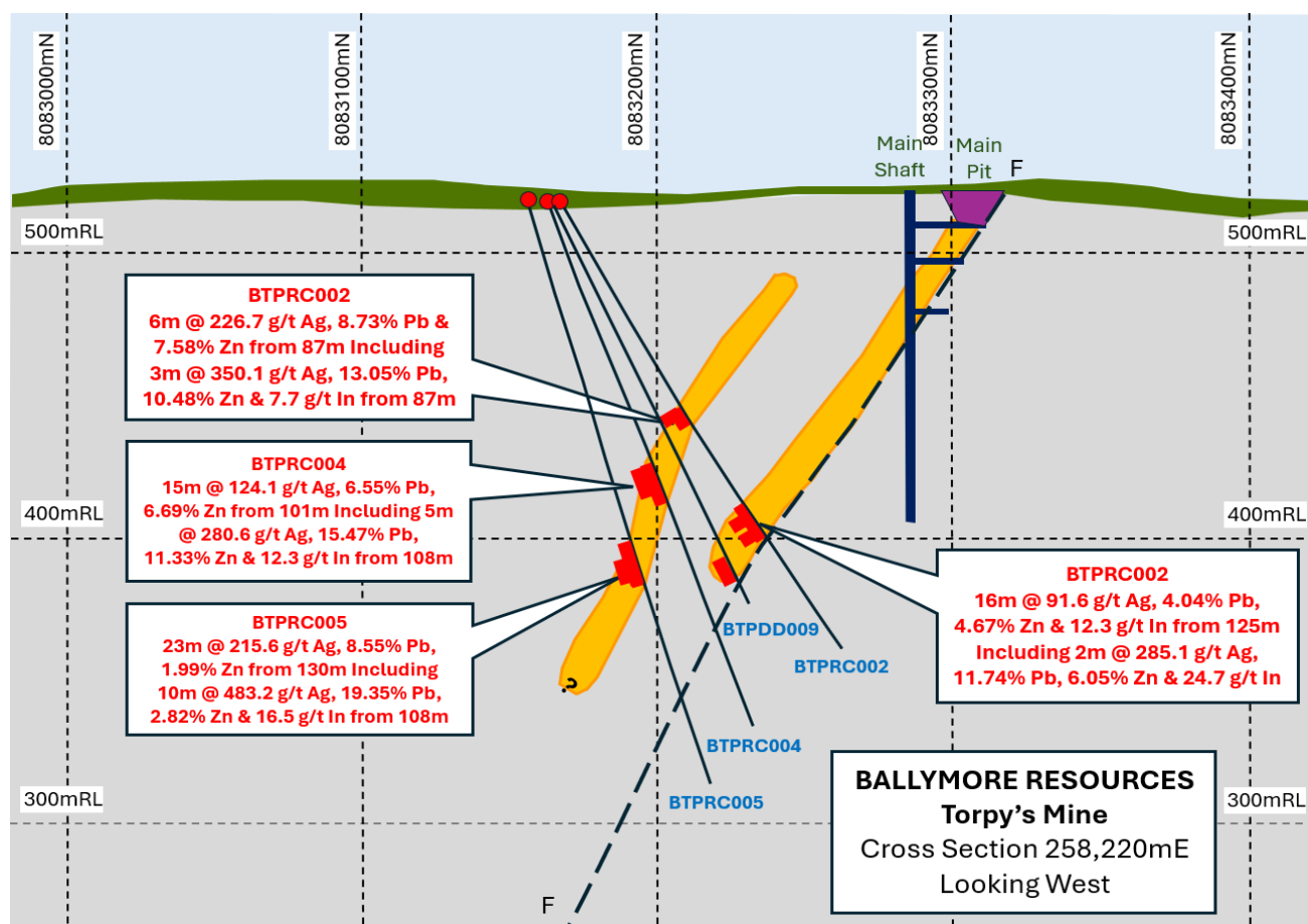
Figure 2 – Torpy's Cross Section 258,220mE looking west, showing historic workings, drill traces massive sulphide lenses.
