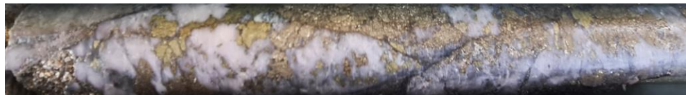
Figure 1 – Drill core from drill Hole DTDD009 showing quartz-chalcopyrite vein material grading 171.8 g/t Au, 56.4 g/t Ag & 5.28% Cu
